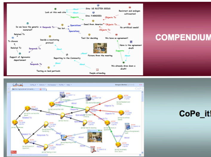
Fig.4. Integration Compendium-CoPe_it!
